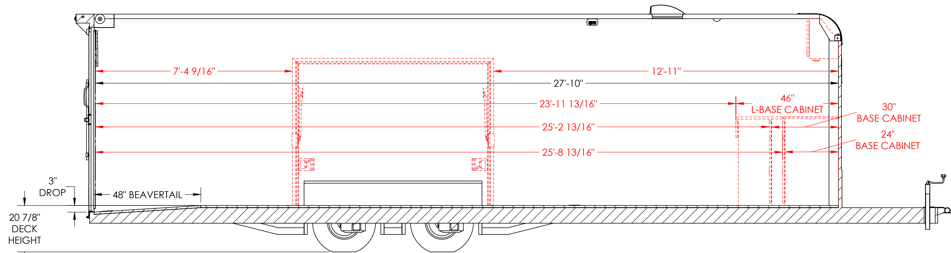
INTERIOR ROAD SIDE SECTION A-A
