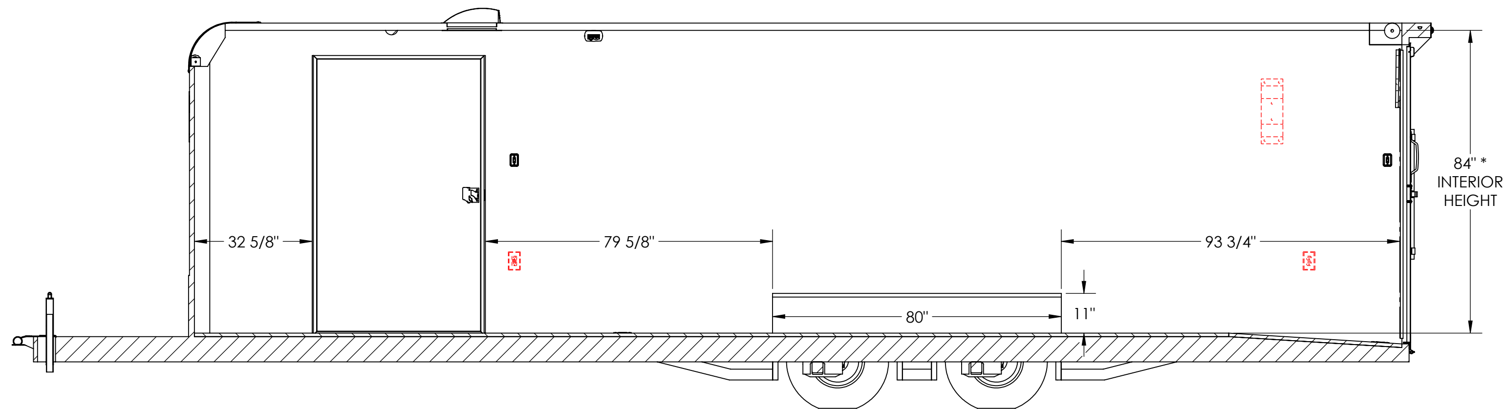
INTERIOR CURB SIDE SECTION B-B
